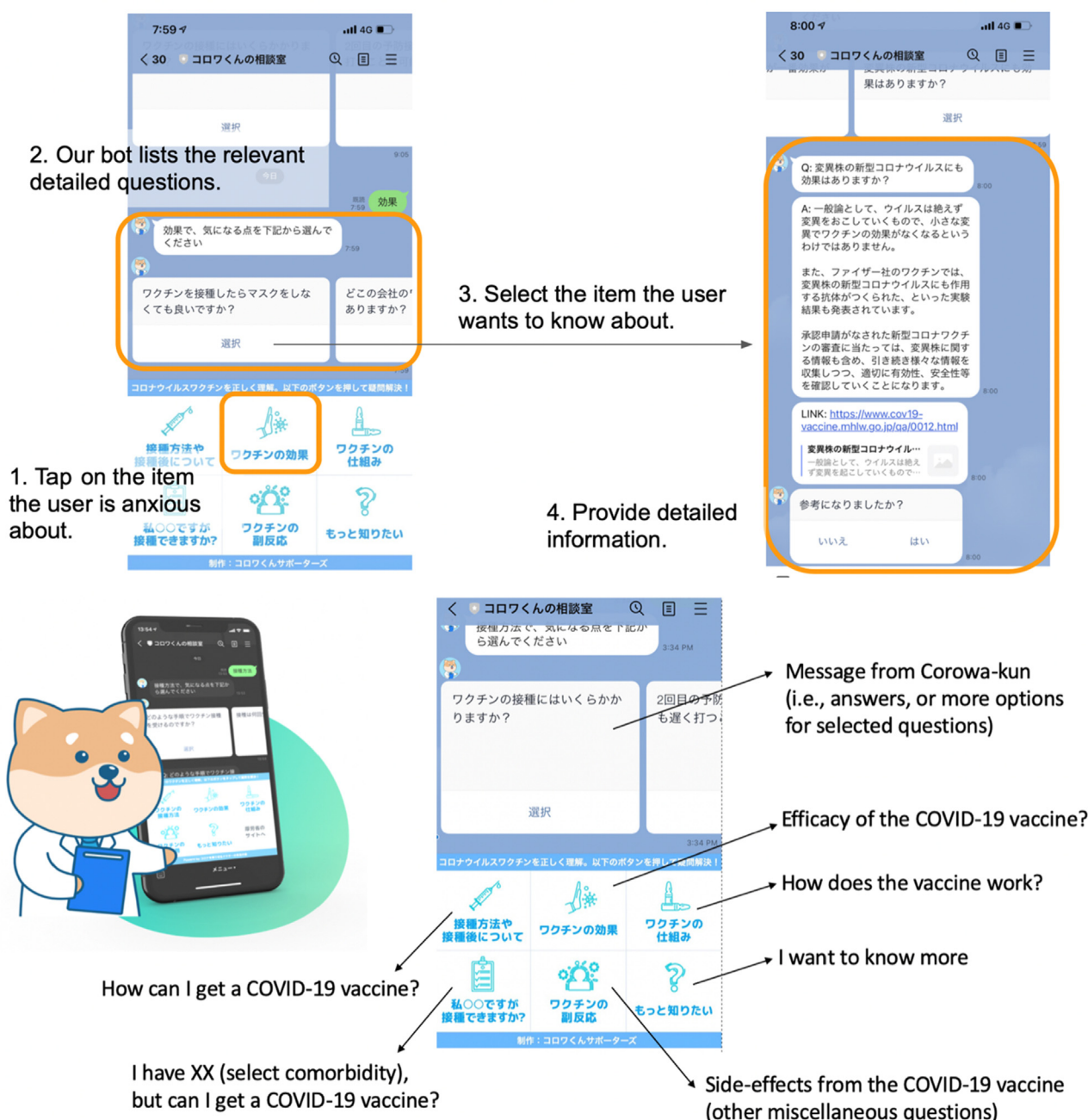
Fig. 1. Corowa-kun's Consultation Room: a free messenger app chatbot, Japan 2021 Corowa-kun is the mascot of an online chatbot. This chatbot in LINE is used to answer COVID-19 vaccine frequently asked questions (FAQs) via text messages. As of May 10th, 70 FAQs are available.
